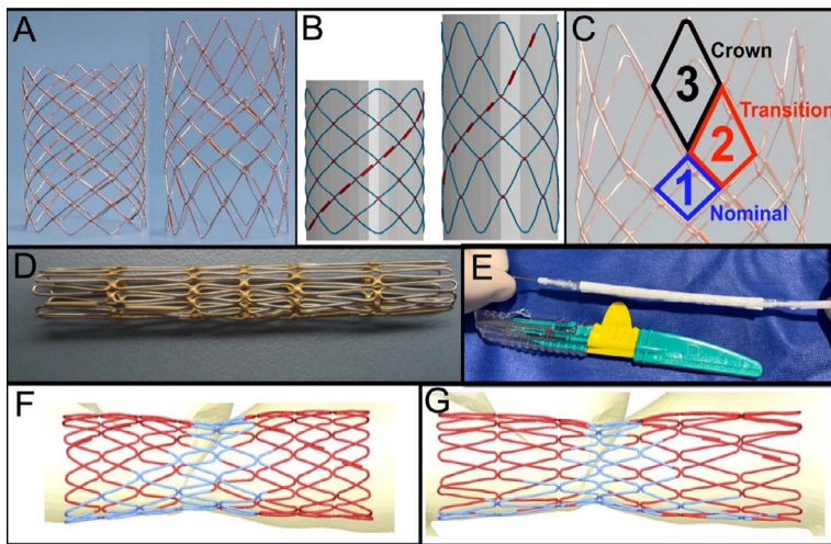
Figure 1 Schematics and photography illustrating the changes made to create the G-ARMOR. Panel A Bare metal 10Zig versions of the original Cheatham-Platinum (CP) stent and the G-ARMOR stent. The difference in shortening between the stents is obvious and illustrated further in schematic panels B and C . Panel C illustrates how changing the length of the wires used to form the distal 2 rows of the stent, creates three different cell morphologies. The originally shaped “nominal” cell (1); the asymmetric “transition” cell (2) and the uniform but larger “crown” cell (3) are marked in panel A , B , C . The modification can also be seen in Panel D , showing a neutral, unboxed bare metal G-ARMOR stent. Panel E shows the covered version of the G-ARMOR, crimped on a BiB balloon and ready to implant. Panels F and G show FEA analysis of an 8Zig version of both the CP Stent, F , and a G-ARMOR, G , stent dilated on the same virtual balloon in the same simulated aortic coarctation. The decreased shortening experienced by the G-ARMOR is readily visible.
